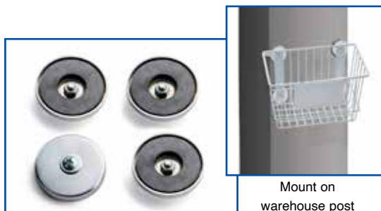
#9904 Magnets 4 pcs. #9902 Magnets 2 pcs. #9901 Magnet 1 pc. (50–60 lb. pull test)
